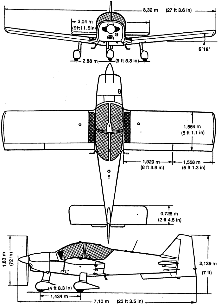
3 View Drawing
