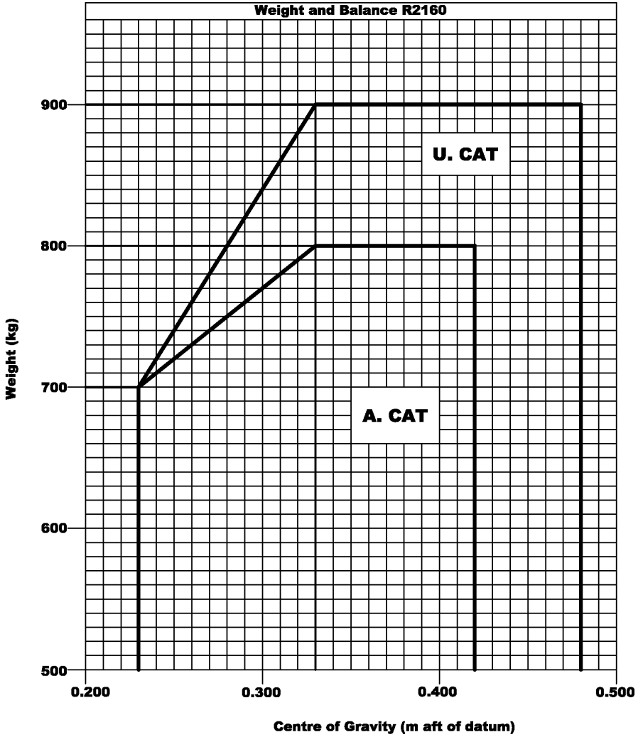
Figure 6-1 Weight and Balance Limits
