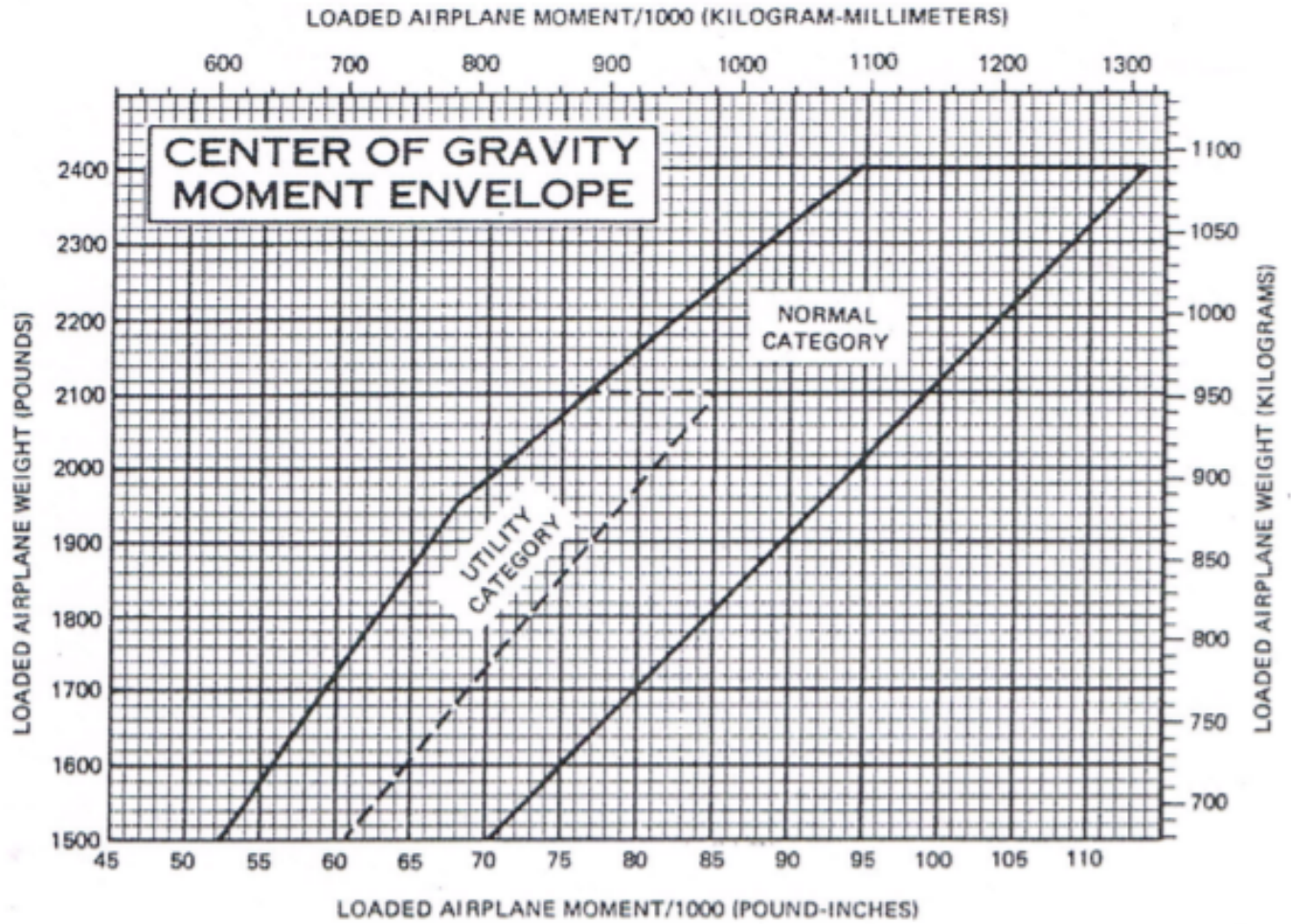
Figure 6-7. Center of Gravity Moment Envelope
